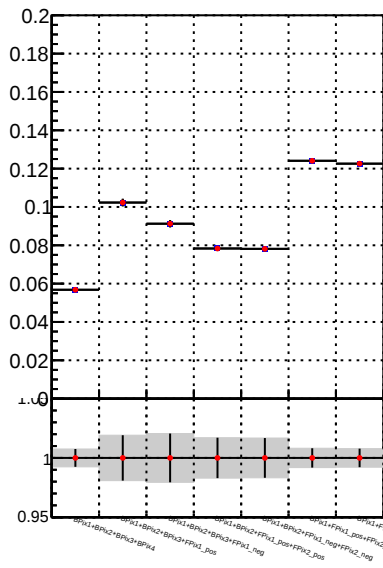
Fake rate vs. DQM_DisplacedSUSY_mkFit DQM_DisplacedSUSY_mkFit_BDT
