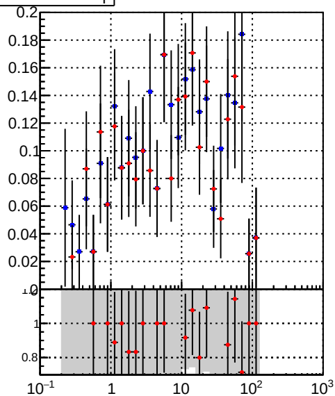
—●— \text{DQM\_DisplacedSUSY\_mkFit\_} —●— \text{DQM\_DisplacedSUSY\_mkFit\_BDT\_}
