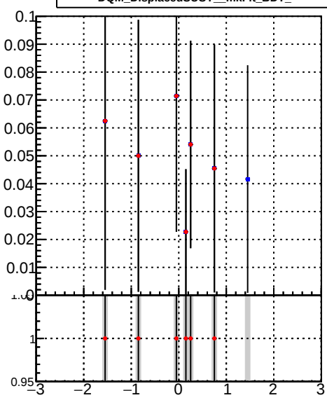
Legend: DQM_DisplacedSUSY_mkFit_ DQM_DisplacedSUSY_mkFit_BDT_
