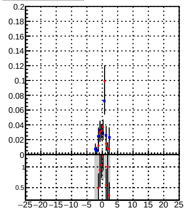
Efficiency vs Dxy(PV) plot
