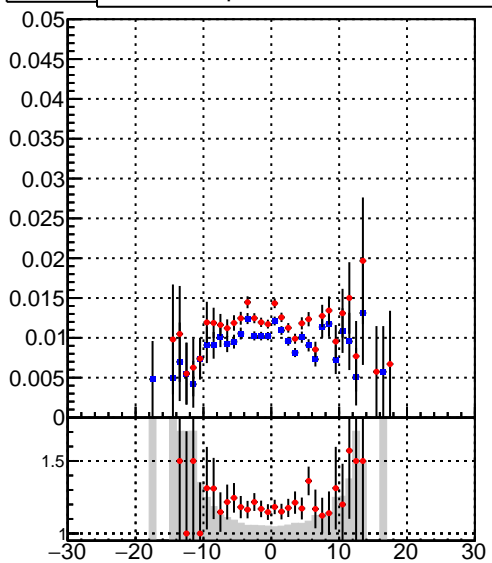
Efficiency vs vert r — DQM_DisplacedSUSY_mkFit_ — DQM_DisplacedSUSY_mkFit_BDT_
