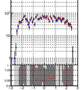
N of reco track vs phi
