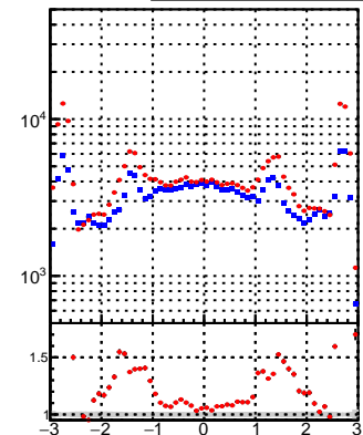
N of reco track vs \eta —•— DQM_DisplacedSUSY_mkFit —x— DQM_DisplacedSUSY_mkFit_BDT_
