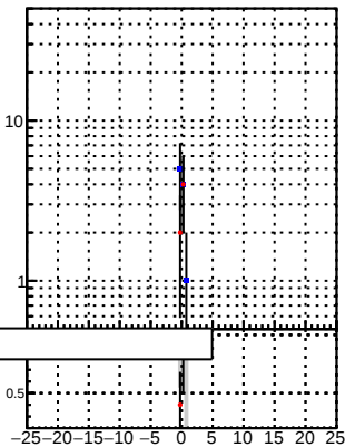
N of associated (recoToSim) loopers tracks vs dxy
