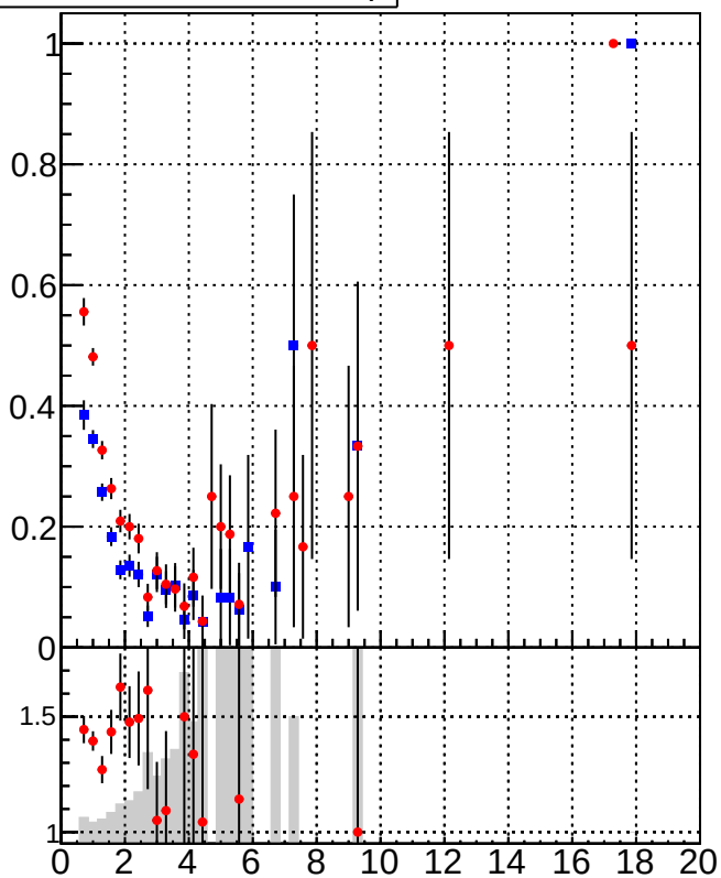
K_S^0 tracking fake rate vs p_T
