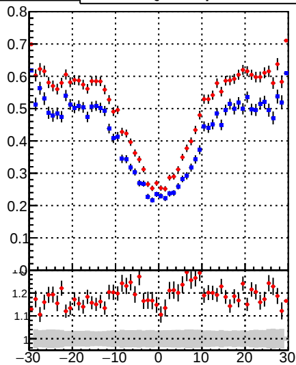
◆ DQM_DisplacedSUSY_mkFit_ × DQM_DisplacedSUSY_mkFit_BDT_
