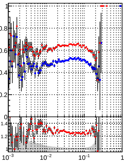
Fake rate vs dr
