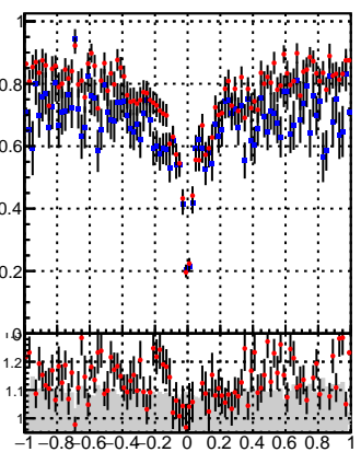
Fake rate vs dx
