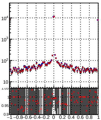
N of sim —●— DQM_DisplacedSUSY__mkFit_BDT__
