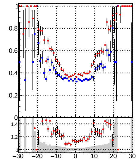
—•— DQM_DisplacedSUSY_mkFit_ —•— DQM_DisplacedSUSY_mkFit_BDT_ Fake rate vs v
