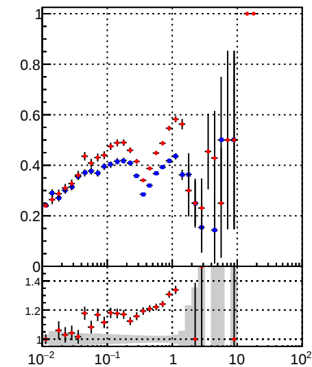
—•— DQM_DisplacedSUSY_mkFit_ —•— DQM_DisplacedSUSY_mkFit_BDT_ Fake rate vs v
