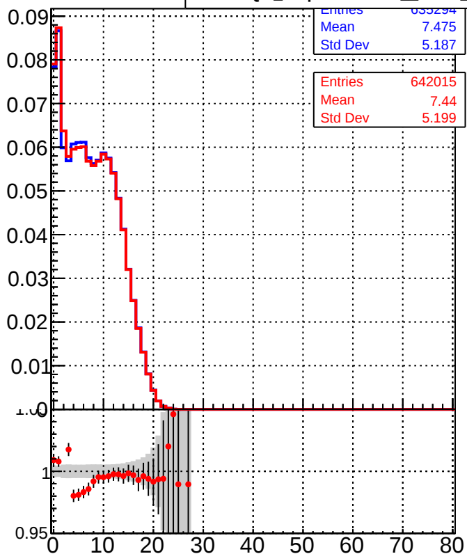
—■— DQM_DisplacedSUSY_mkFit_ —●— DQM_DisplacedSUSY_mkFit_BDT_
