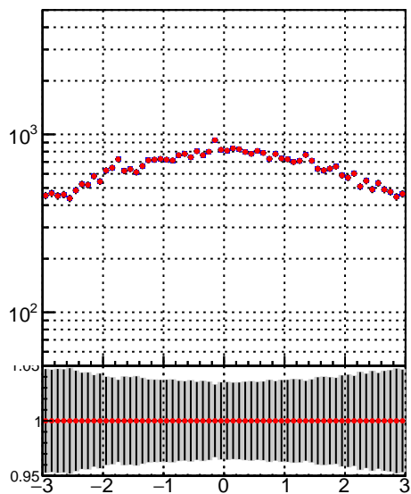
Legend for the plots: Blue star: DQM_DisplacedSUSY_mkFit_ Red star: DQM_DisplacedSUSY_mkFit_BDT_
