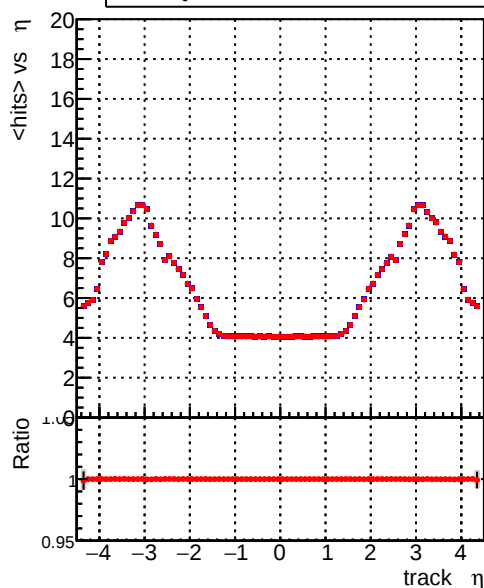
mean hits vs \eta Legend: DQM_mkFitFitnit_noSel (blue line), DQM_mkFitFitnit_noSel (red line)
