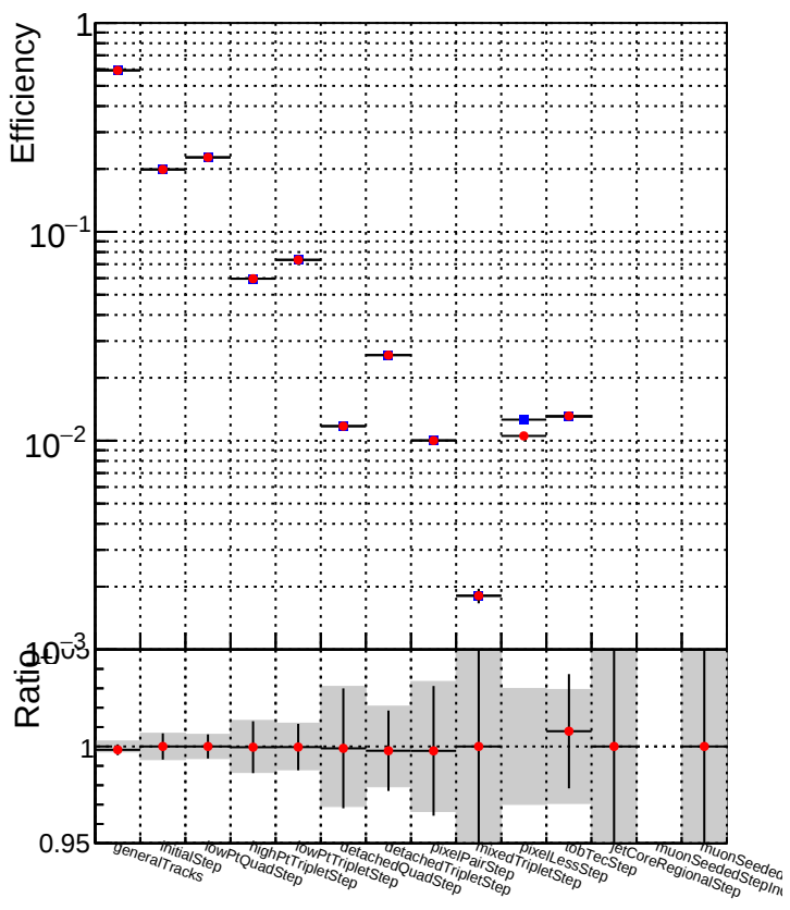
DQM_V0001_R000000001_Global_mkFitbase_RECO DQM_V0001_R000000001_Global_CMSSW_X_Y_Z_RECO
