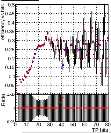
DQM_V0001_R000000001_Global_mkFitbase_RECO Efficiency DQM_V0001_R000000001_Global_CMSSW_X_Y_Z_RECO
