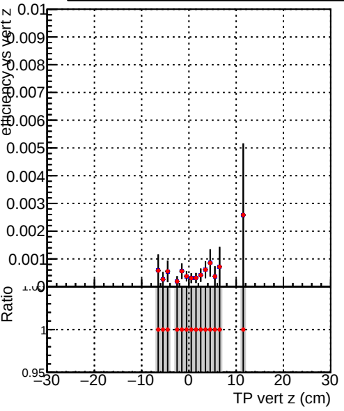
Efficiency vs vertpos Legend: DQM_V0001_R0000000001_Global_mkFitbase_RECO DQM_V0001_R0000000001_Global_CMSSW_X_Y_Z_RECO
