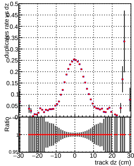
al__mkFitbase__RECO al__CMSSW_X_Y_Z__RECO
