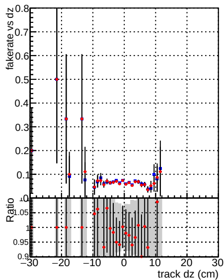
DQM_V0001_R000000001_Global_mkFitbase_RECO Fake rate vs d DQM_V0001_R000000001_Global_CMSSW_X_Y_Z_RECO
