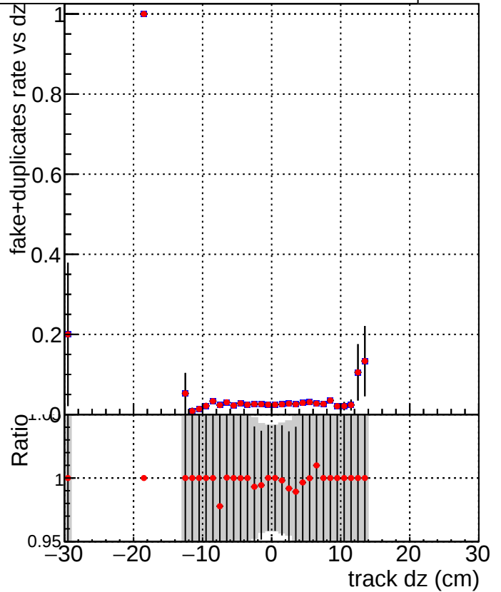
fake+duplicates rate vs dz
