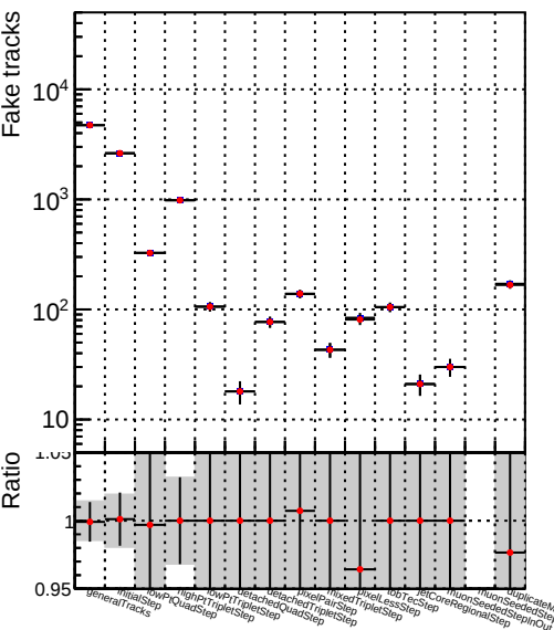
Number —●— DQM_V0001_R000000001_Global_CMSSW_X_Y_Z_RECO
