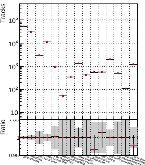
DQM_V0001_R000000001_Global_mkFitbase_RECO
