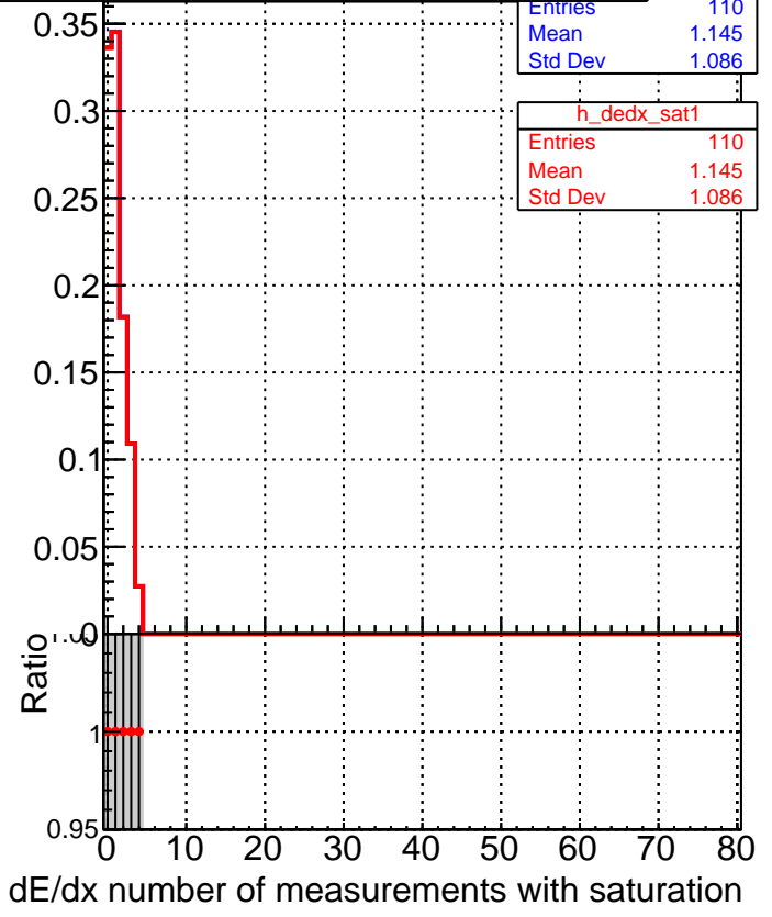
■ DQM_V0001_R000000001_Global_mkFitbase_RECO ● DQM_V0001_R000000001_Global_CMSSW_X_Y_Z_RECO
