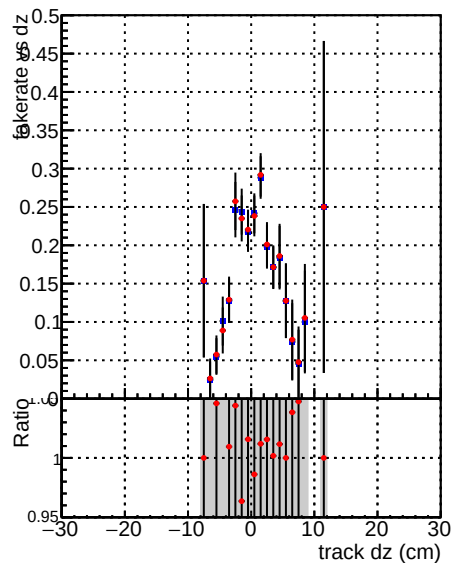
Fake rate vs dz Legend: Global mkFitbase RECO (Blue line with dots) Global mCSSLW X Y Z RECO (Red line with dots)
