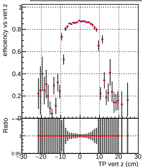
—●— DQM_V0001_R000000001_Global_mkFitbase_RECO —●— DQM_V0001_R000000001_Global_CMSSW_X_Y_Z_RECO
