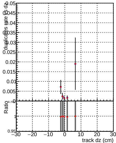
Global mkFitbase RECO —●— DQM V0001_R0000000001 —●— DQM V0001_R0000000001 Global CMSSW X Y Z RECO
