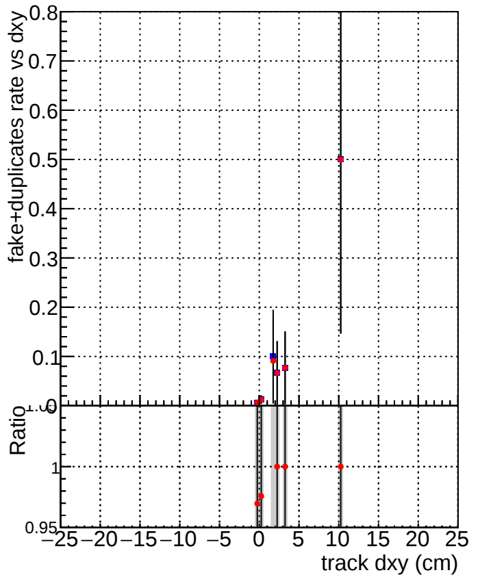
DQM_V0001_R000000001_Global_mkFitbase_RECO DQM_V0001_R000000001_Global_CMSSW_X_Y_Z_RECO
