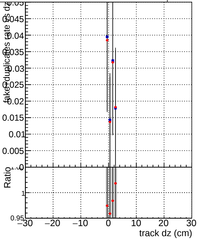
DQM_V0001_R000000001_Global_mkFitbase_RECO DQM_V0001_R000000001_Global_CMSSW_X_Y_Z_RECO
