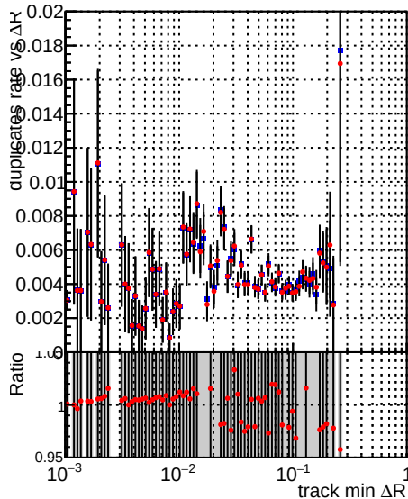
—•— DQM_V0001_R000000001_Global_mkFitbase_RECO —•— DQM_V0001_R000000001_Global_CMSSW_X_Y_Z_RECO
