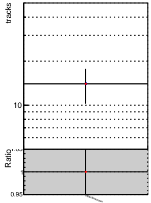
DQM_V0001_R000000001_Global_mkFitbase_RECO DQM_V0001_R000000001_Global_CMSSW_X_Y_Z_RECO
