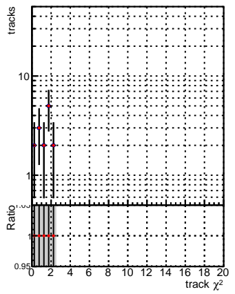
DQM_V0001_R000000001_Global_mkFitbase_RECO DQM_V0001_R000000001_Global_CMSSW_X_Y_Z_RECO
