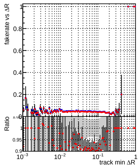
—●— DQM_V0001_R000000001_Global_mkFitbase_RECO —●— DQM_V0001_R000000001_Global_CMSSW_X_Y_Z_RECO
