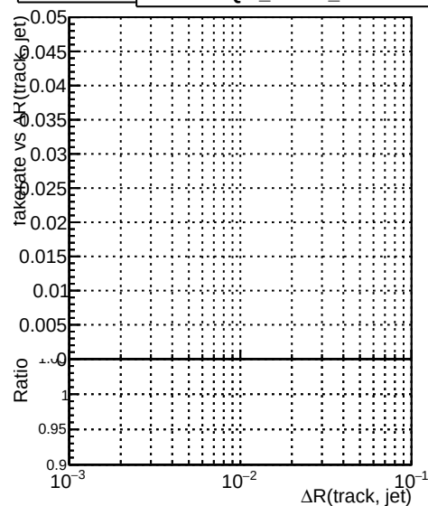
—●— DQM_V0001_R000000001_Global_mkFitbase_RECO —●— DQM_V0001_R000000001_Global_CMSSW_X_Y_Z_RECO
