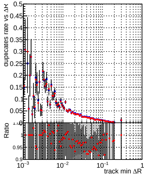
—●— DQM_V0001_R000000001_Global_mkFitbase_RECO —●— DQM_V0001_R000000001_Global_CMSSW_X_Y_Z_RECO
