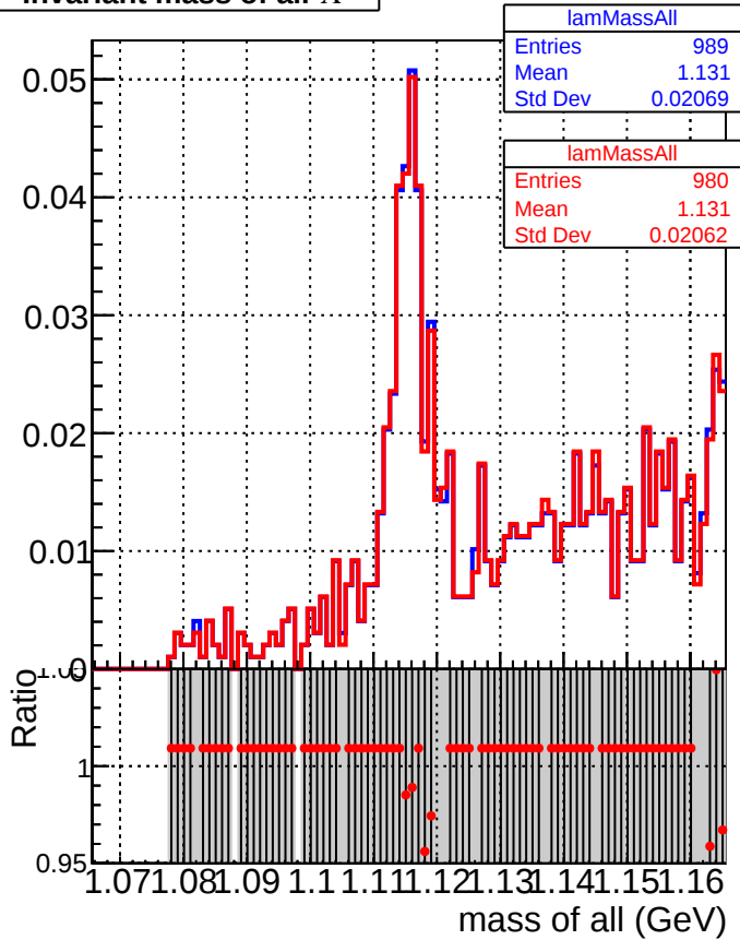
Invariant mass of all \Lambda^0
