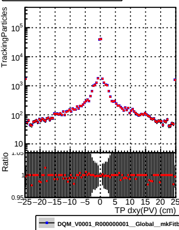
N of sim DQM_V0001_R000000001_Global_CMSSW_X_Y_Z_RECO
