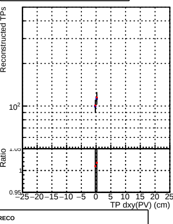
N of associated tracks (simToReco) vs dxy(PV)
