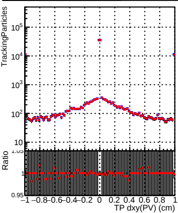
N of sim DQM_V0001_R000000001_Global_CMSSW_X_Y_Z_RECO
