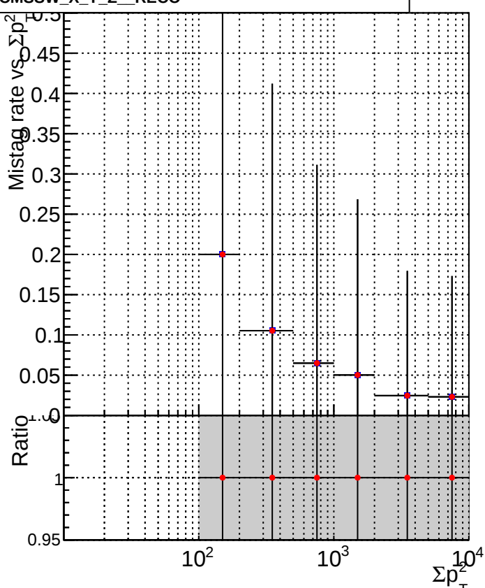
DQM_V0001_R000000001_Global_mkFitbase_RECO DQM_V0001_R000000001_Global_CMSSW_X_Y_Z_RECO
