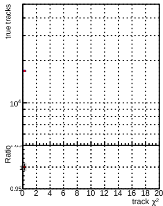
1__Global__CMSSW_X_Y_Z__RECO
