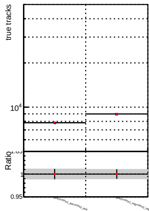
1__Global__CMSSW_X_Y_Z__RECO
