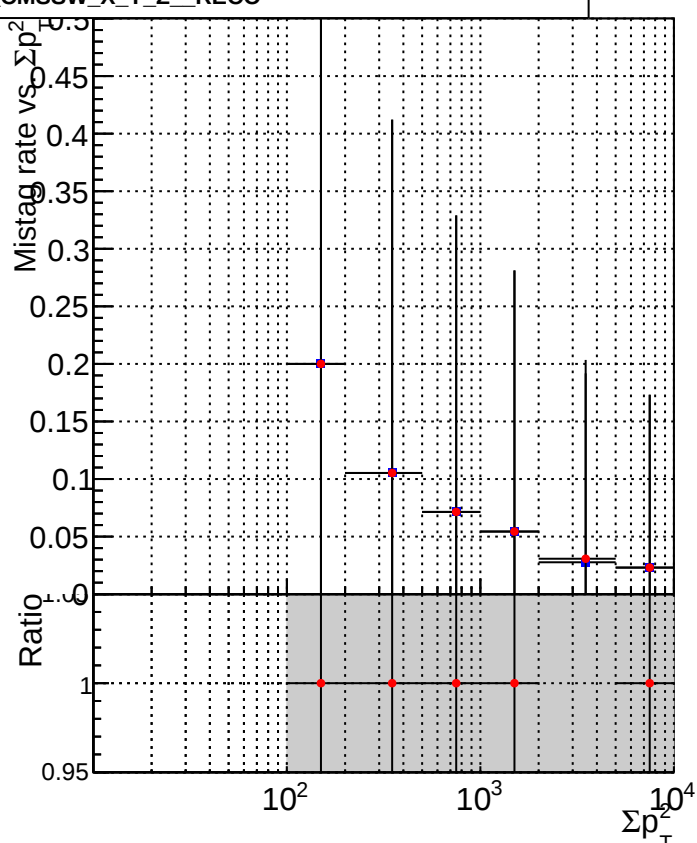
—■ DQM_V0001_R000000001_Global_mkFitbase_RECO —● DQM_V0001_R000000001_Global_CMSSW_X_Y_Z_RECO
