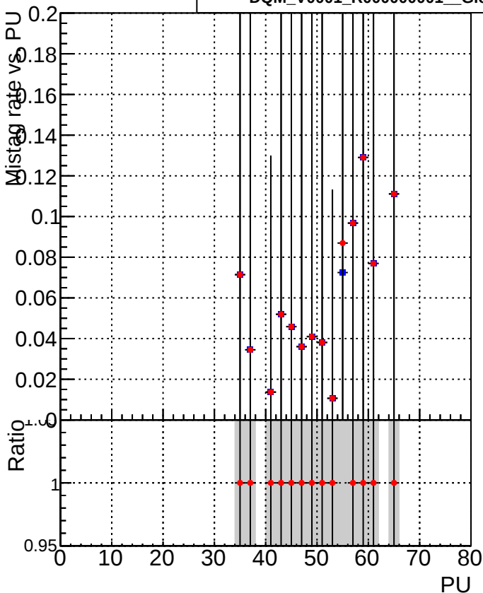
—■ DQM_V0001_R000000001_Global_mkFitbase_RECO —● DQM_V0001_R000000001_Global_CMSSW_X_Y_Z_RECO
