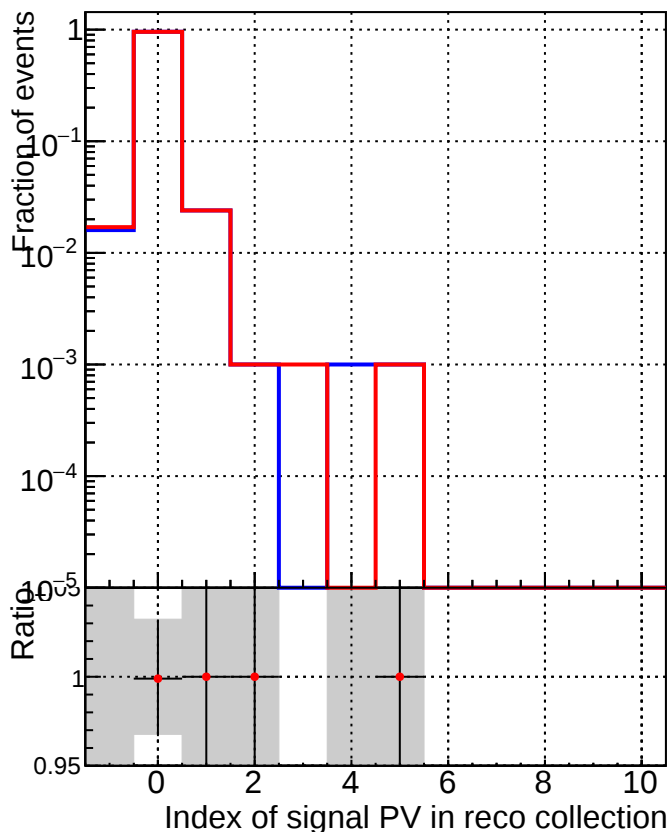
—■ DQM_V0001_R000000001_Global_mkFitbase_RECO —● DQM_V0001_R000000001_Global_CMSSW_X_Y_Z_RECO
