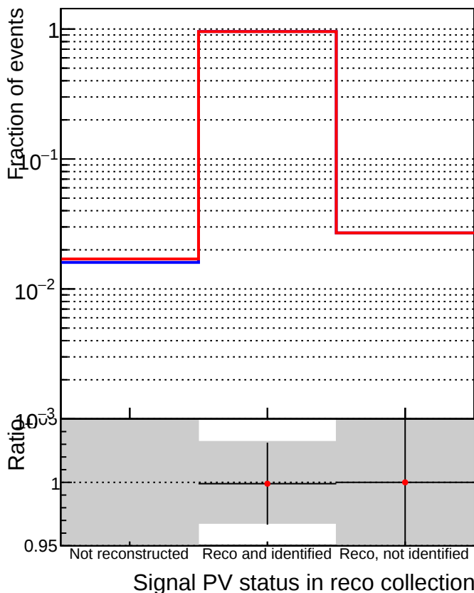
—■ DQM_V0001_R000000001_Global_mkFitbase_RECO —● DQM_V0001_R000000001_Global_CMSSW_X_Y_Z_RECO
