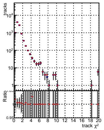
N of reco track vs. - DQM_V0001_R000000001_Global_mkFitbase_RECO - DQM_V0001_R000000001_Global_CMSSW_X_Y_Z_RECO
