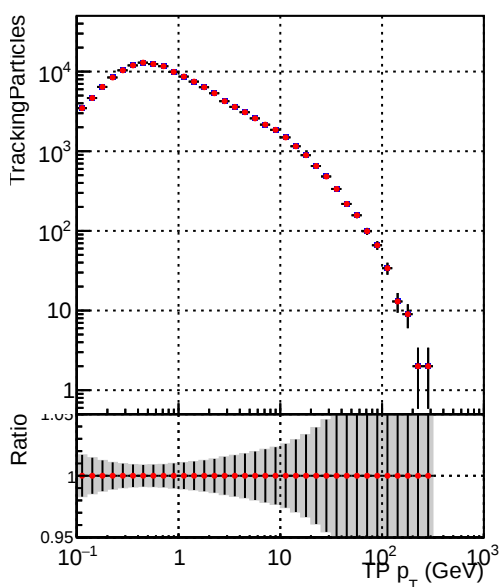
—•— DQM_V0001_R000000001_Global_mkFitbase_RECO —•— DQM_V0001_R000000001_Global_CMSSW_X_Y_Z_RECO
