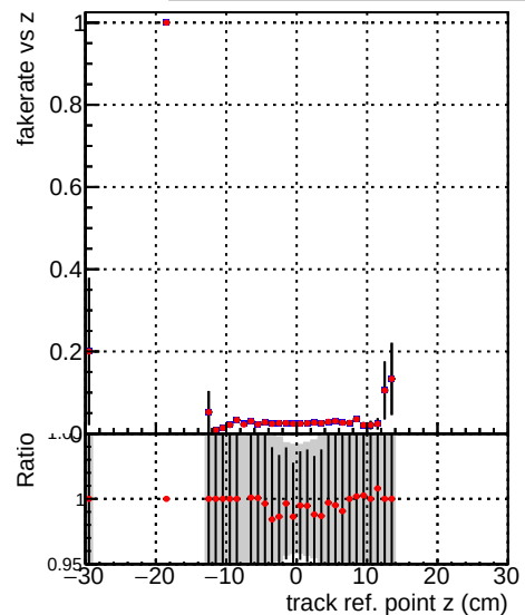
Fake rate vs verpos Legend: —•— DQM_V0001_R000000001_Global_mkFitbase_RECO —•— DQM_V0001_R000000001_Global_CMSSW_X_Y_Z_RECO
