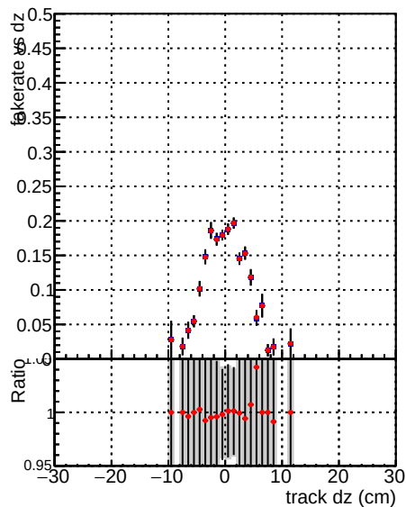
DQM V0001_R000000001 Global mkFitbase RECO Fake rate vs d —●— —●— —●— —●— Duplicates Rate vs Dxy —●— —●— —●— —●— Pileup rate vs dxy —●— —●— —●— —●—
