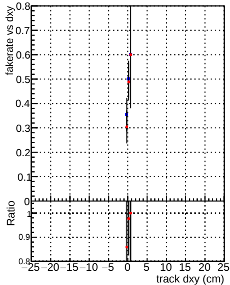
DQM V0001_R000000001 Global mkFitbase RECO Fake rate vs d Blue dots Red dots Black line Grey line Duplicates Rate vs Dxy Blue dots Red dots Black line Grey line Pileup rate vs dxy Blue dots Red dots Black line Grey line
