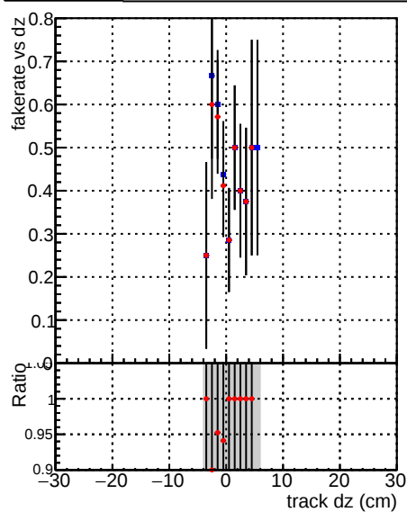
DQM V0001_R000000001 Global mkFitbase RECO Fake rate vs d Blue dots Red dots Black line Grey line Duplicates Rate vs Dxy Blue dots Red dots Black line Grey line Pileup rate vs dxy Blue dots Red dots Black line Grey line
