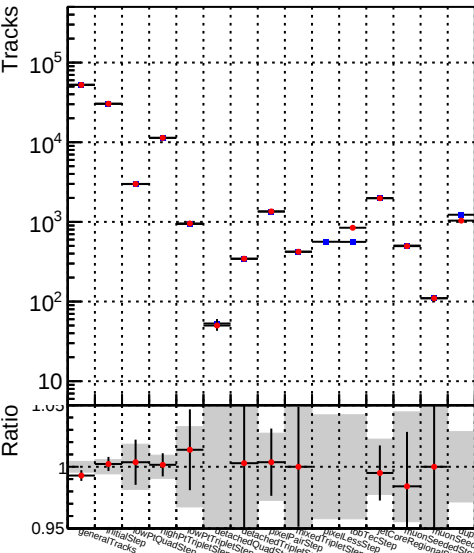
DQM_V0001_R000000001_Global_mkFitbase_RECO
