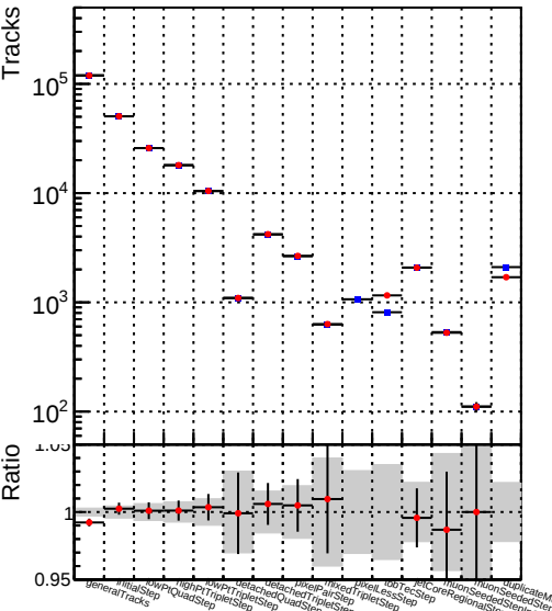
DQM_V0001_R000000001__Global__mkFitbase__RECO
