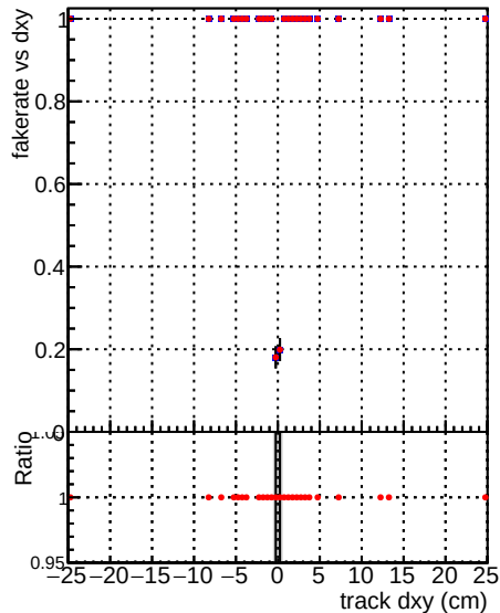
Global mkFitbase RECO Fake rate vs d DQM_V0001_R0000000001 DQM_V0001_R0000000001 DQM_V0001_R0000000001 Duplicates Rate vs Dxy DQM_V0001_R0000000001 DQM_V0001_R0000000001 DQM_V0001_R0000000001 Pileup rate vs dxy DQM_V0001_R0000000001 DQM_V0001_R0000000001 DQM_V0001_R0000000001
