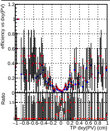
Efficiency vs Dxy(PV) DQM_V0001_R000000001_Global_mkFitbase_RECO DQM_V0001_R000000001_Global_CMSSW_X_Y_Z_RECO
