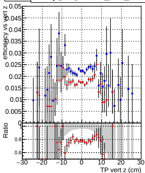
Efficiend —●— DQM_V0001_R000000001_Global_CMSSW_X_Y_Z_RECO
