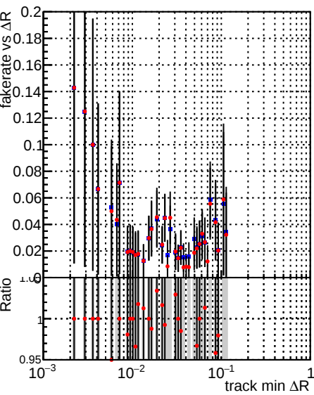
Fake rate vs \Delta R(\text{track, jet}) Legend: DQM_V0001_R000000001_Global_mkFitbase_RECO (blue), DQM_V0001_R000000001_Global_CMSSW_X_Y_Z_RECO (red)
