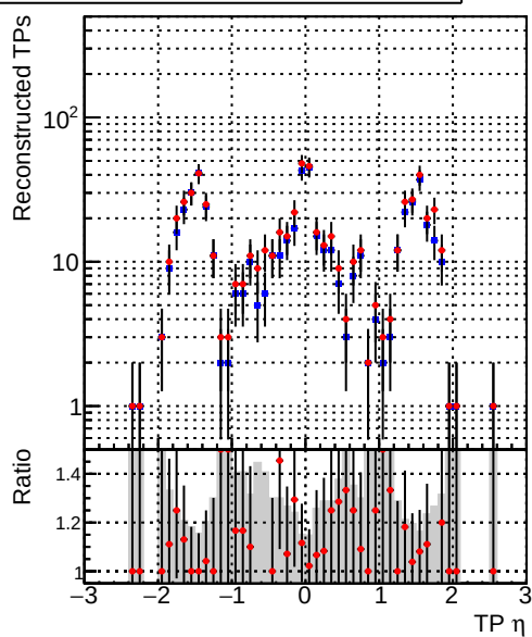
—•— DQM_V0001_R000000001_Global_mkFitbase_RECO —•— DQM_V0001_R000000001_Global_CMSSW_X_Y_Z_RECO
