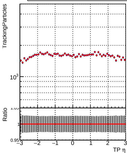
—•— DQM_V0001_R000000001_Global_mkFitbase_RECO —•— DQM_V0001_R000000001_Global_CMSSW_X_Y_Z_RECO
