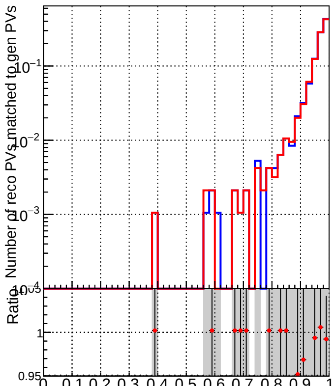
RecoPVAssoc2GenPVMatched_Purity
